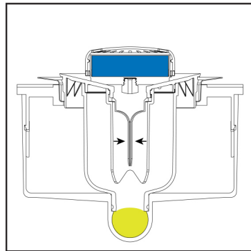
3. After liquid has passed, elastomer trap seals to prevent escape of malodor.
